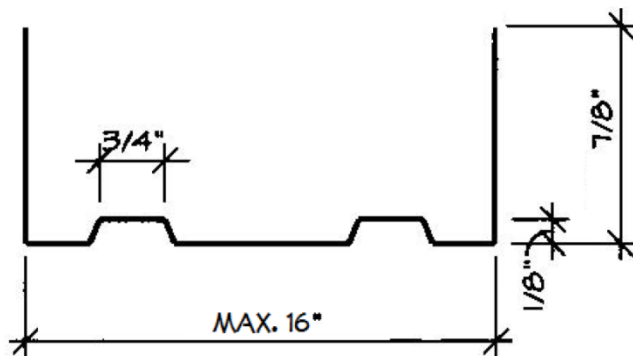
U Panel Dimensions
